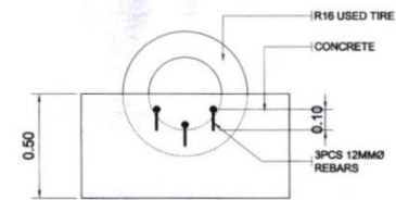
SECTION / ELEVATION
