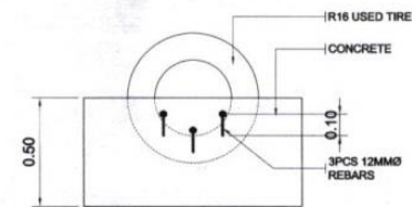
SECTION / ELEVATION
