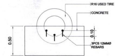
SECTION / ELEVATION
