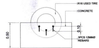
SECTION / ELEVATION
